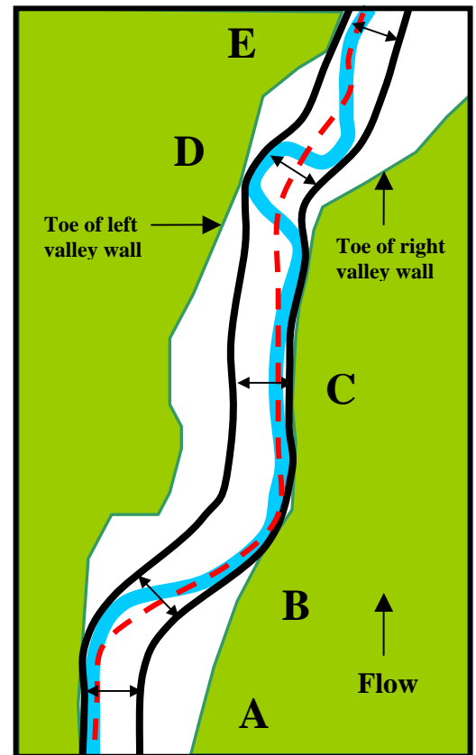
Figure 5. River corridor drawn for a reach of river straightened against the toe of the valley.
