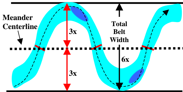
Figure 4. Idealized representation of a river corridor drawn to accommodate the meander belt width, measured out as parallel lines “3 x channel width” either side a meander centerline drawn down valley through the crossover or inflection points of the river (dotted line).
