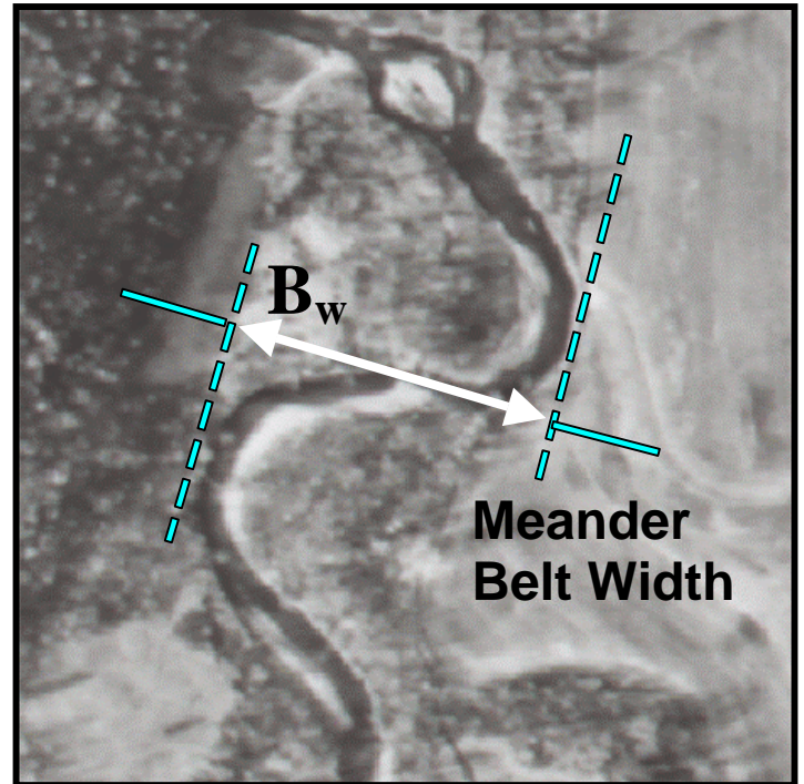
Figure 1. Meander Belt Width ( B_w ) defined by the lateral extent of meanders when the channel slope is in equilibrium with the sediment transport requirements of the river.
